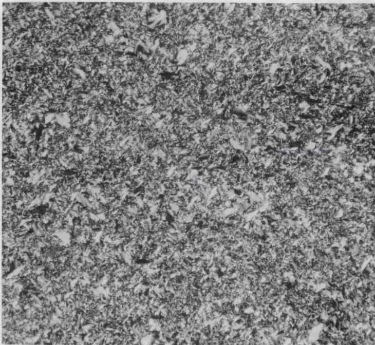
FIGURE 25. PHOTOMICROGRAPHS OF BERYLLIUM COLD HYDROSTATICALLY EXTRUDED AT A RATIO OF 4:1 THROUGH BATTELLE'S DOUBLE-REDUCTION DIE
